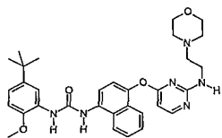
1-(5-tert-Butyl-2-methoxy-phenyl)-3-{4-[2-(2-morpholin-4-yl-ethyl-amino)-pyrimidin-4-yloxy]-naphthalen-1-yl}-urea;
